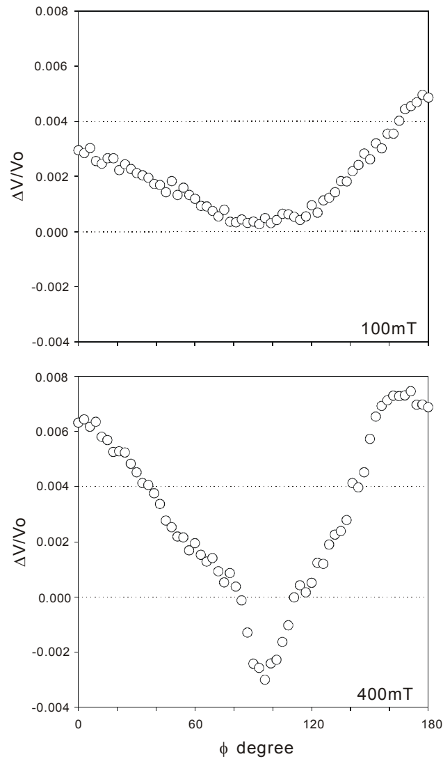
Figure 7. Anisotropy of the ultrasonic propagation velocity (4MHz)
