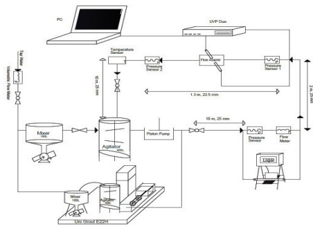
Figure 1 Schematic illustration of the flow loop used for field like conditions
